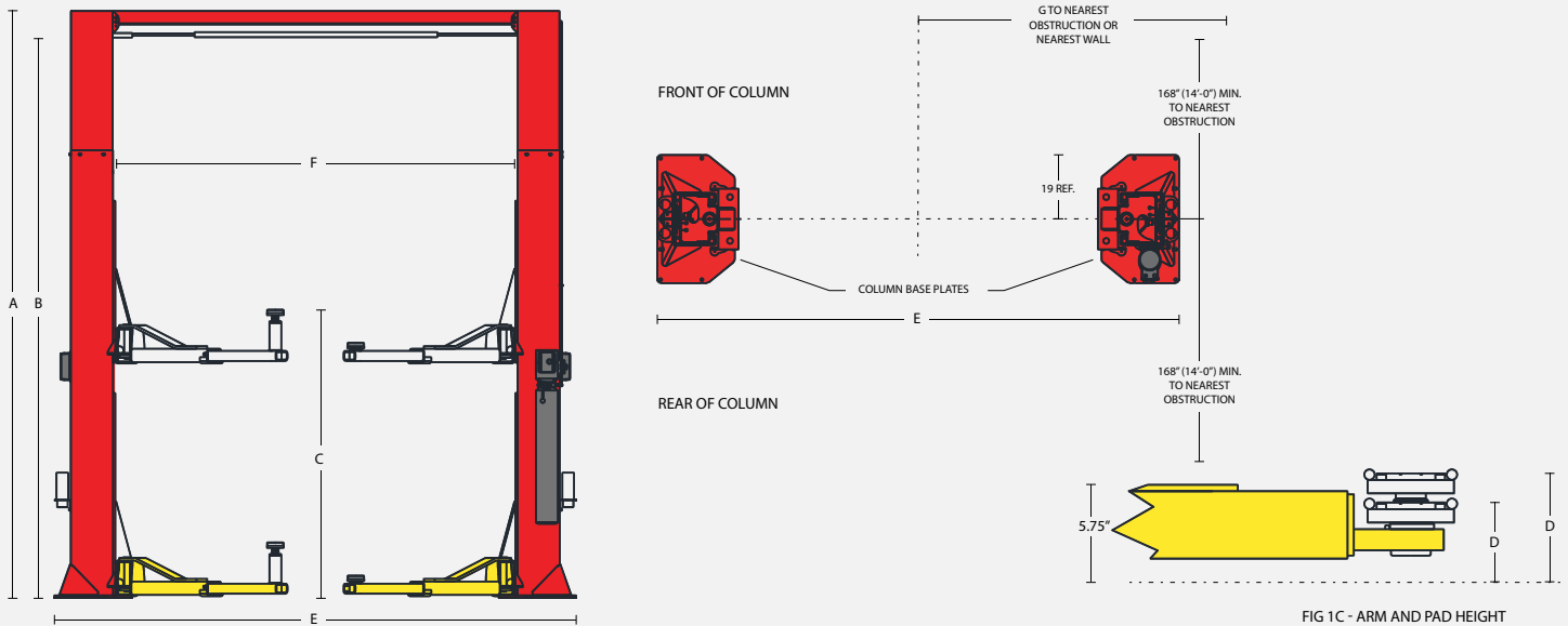
FIG 1C - ARM AND PAD HEIGHT w/o STACK ADAPTERS
